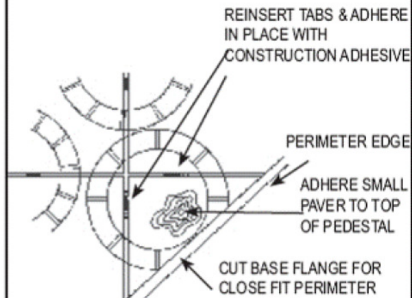
TOP VIEW OF PEDESTAL
