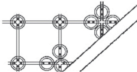
ENLARGED PLAN VIEW AT DIAGONAL PERIMETER EDGE
