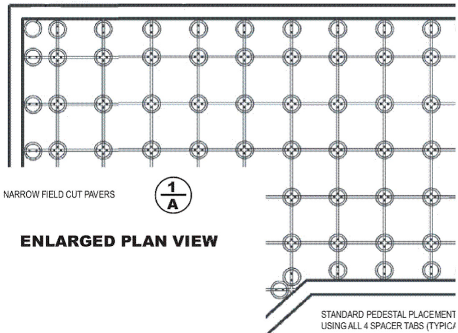
ENLARGED PLAN VIEW AT DIAGONAL PERIMETER EDGE
