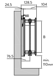
TYPE 22-PKKP
