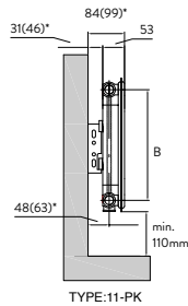
TYPE 11-PK
