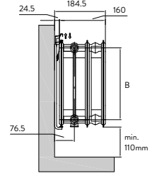
TYPE 33-PKKPKP
