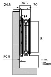
TYPE 21-PKP
